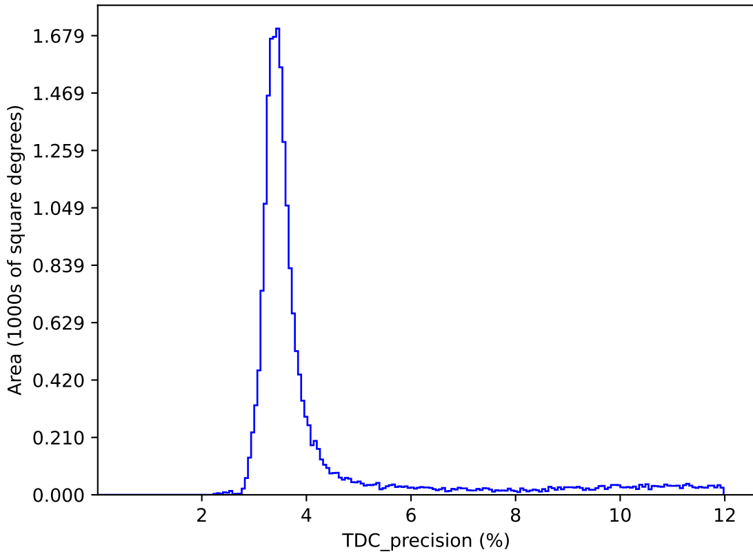
noroll_v3.4_10yrs : TDC_precision
