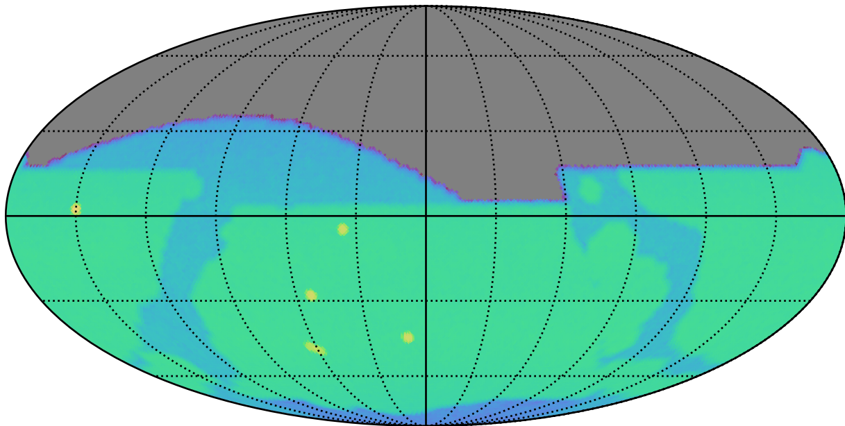
noroll_v3.4_10yrs i: SurfaceBrightLimit
