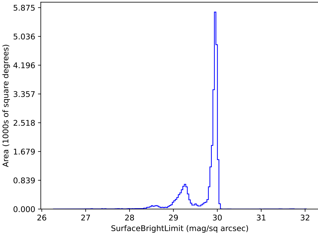
noroll_v3.4_10yrs i: SurfaceBrightLimit
