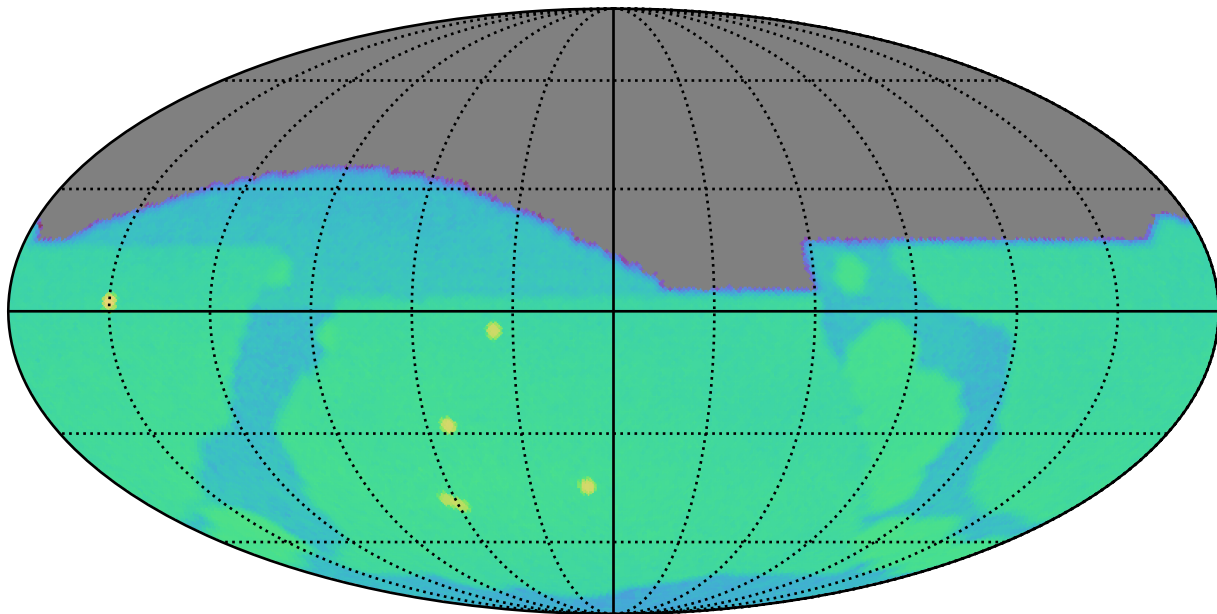
noroll_v3.4_10yrs g: SurfaceBrightLimit
