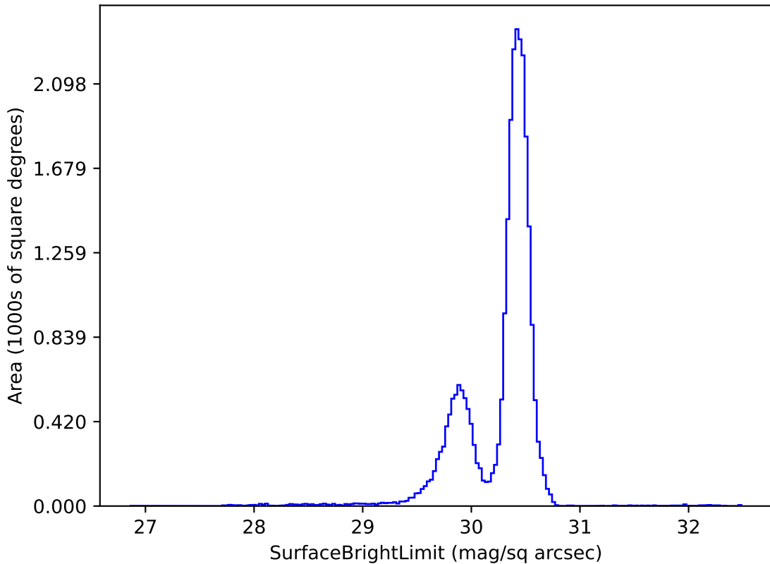
noroll_v3.4_10yrs g: SurfaceBrightLimit
