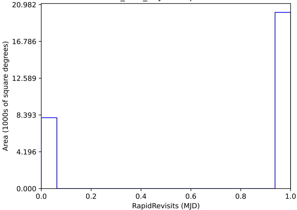
noroll_v3.4_10yrs : RapidRevisits
