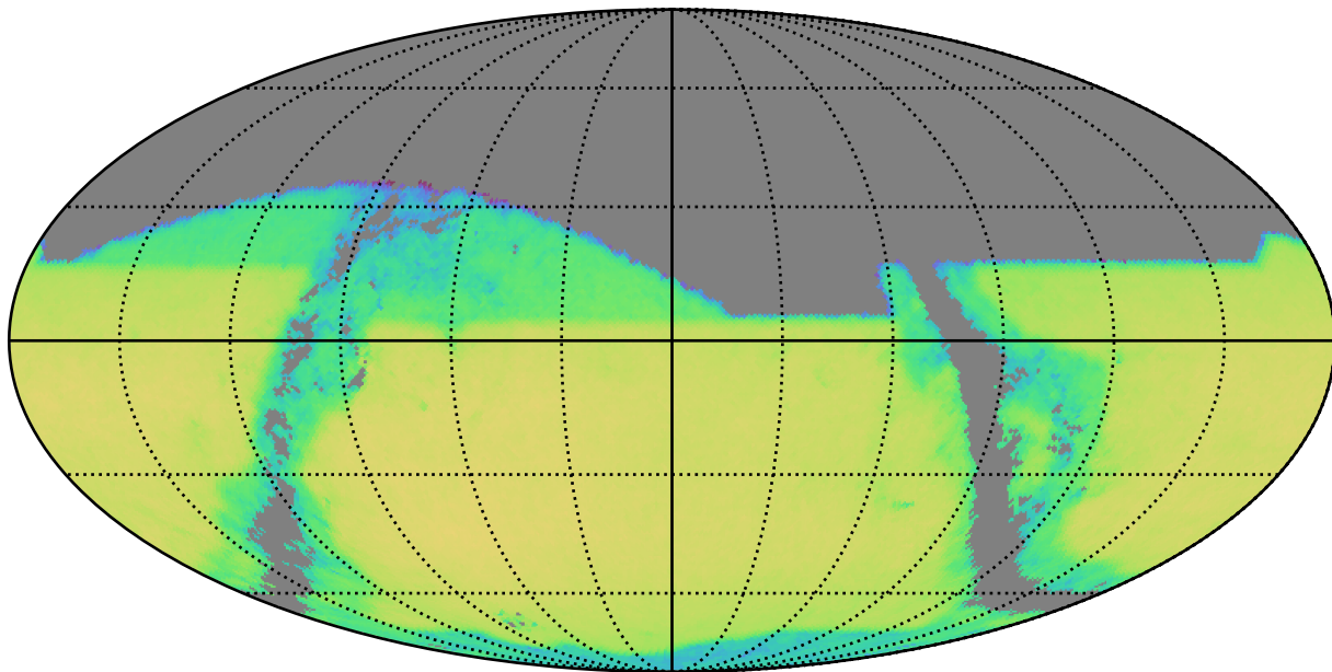
noroll_v3.4_10yrs z band and non-DD: QSONumberCountsMetric
