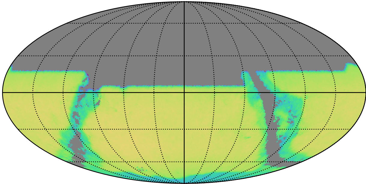
noroll_v3.4_10yrs y band and non-DD: QSONumberCountsMetric
