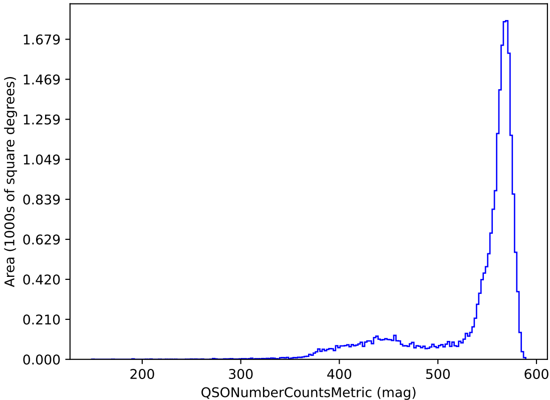
noroll_v3.4_10yrs y band and non-DD: QSONumberCountsMetric
