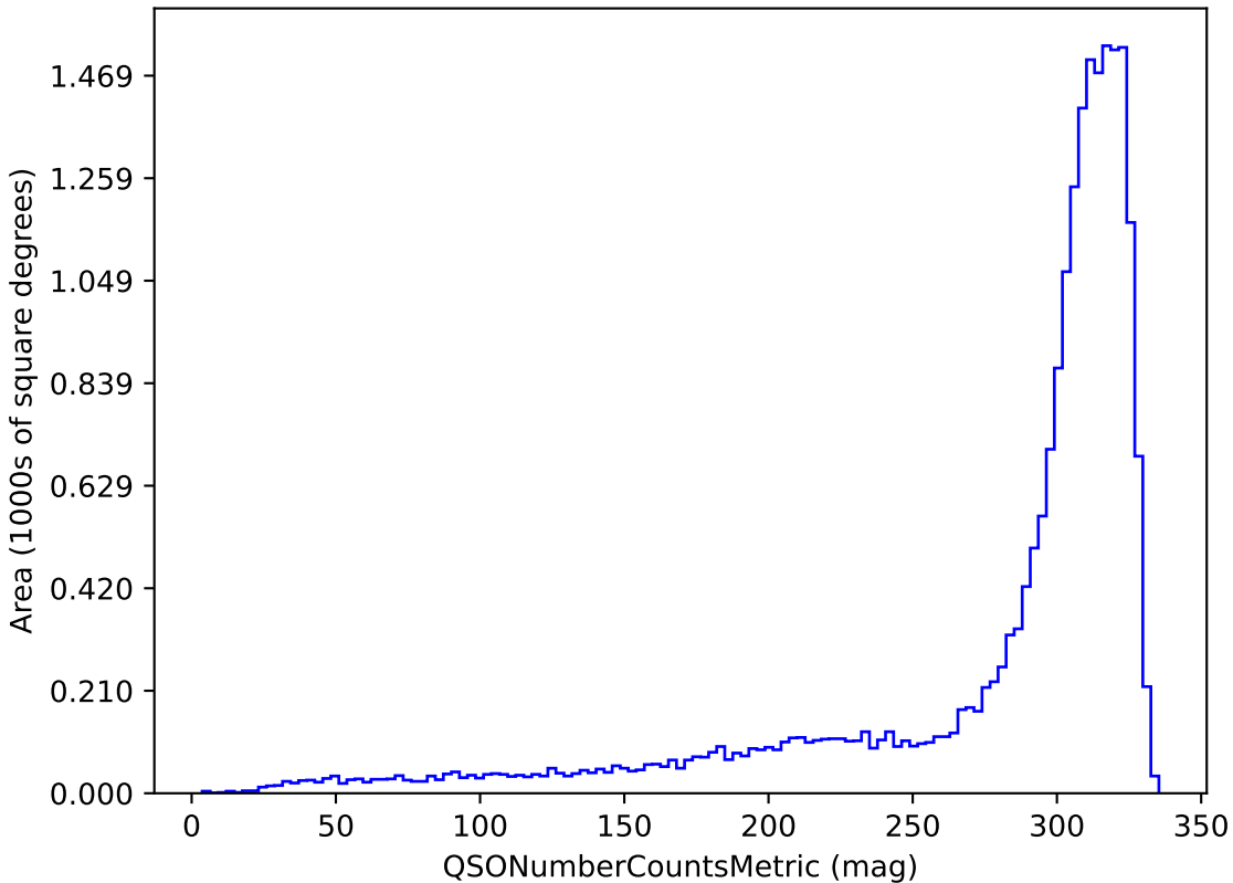
noroll_v3.4_10yrs u band and non-DD: QSONumberCountsMetric
