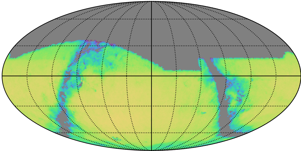
noroll_v3.4_10yrs g band and non-DD: QSONumberCountsMetric
