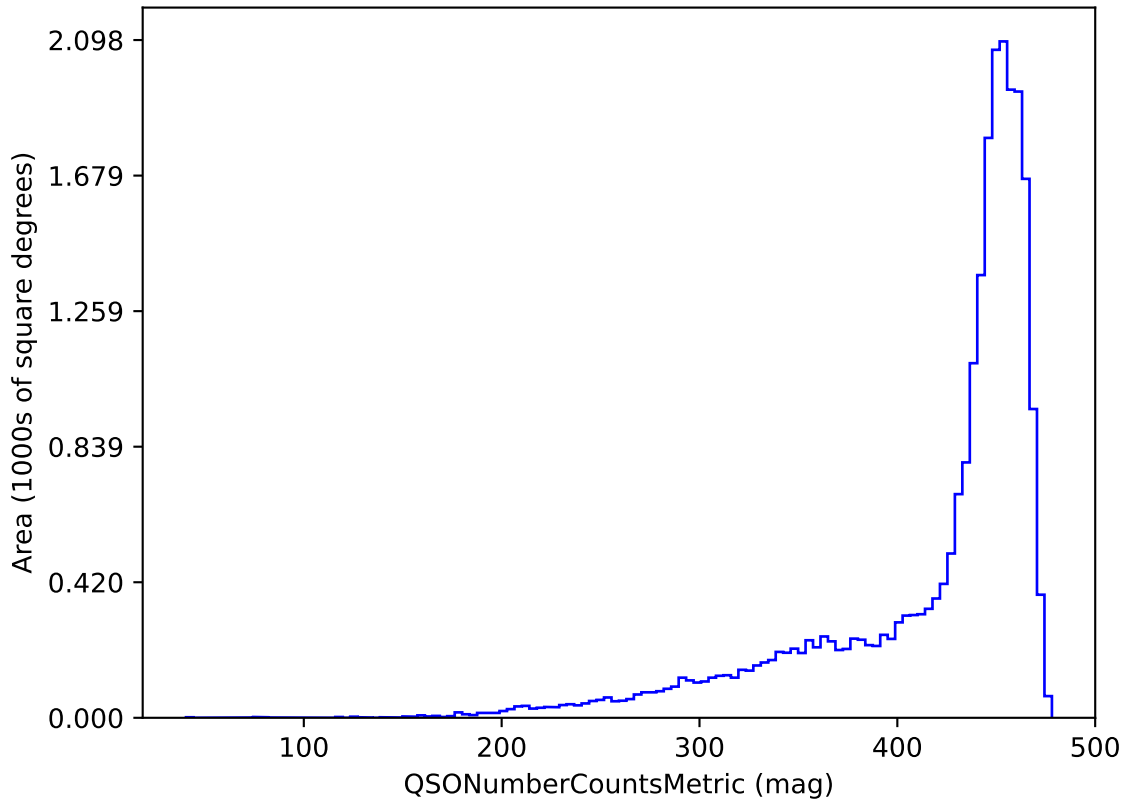
noroll_v3.4_10yrs g band and non-DD: QSONumberCountsMetric
