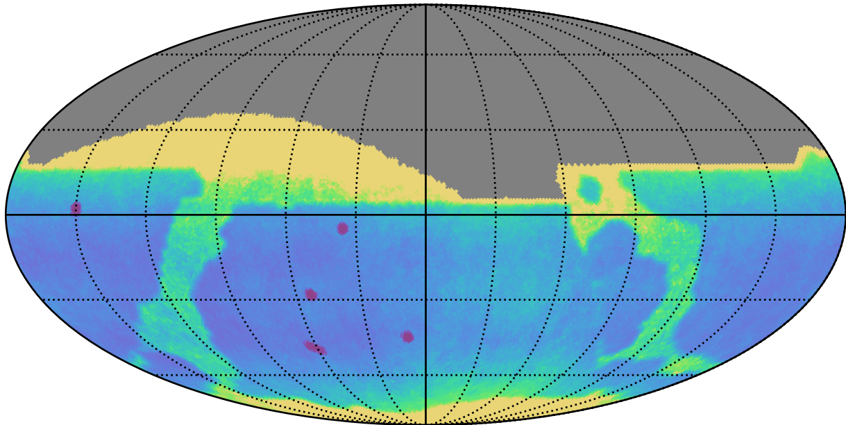
noroll_v3.4_10yrs : Proper Motion Uncert @ 24.0
