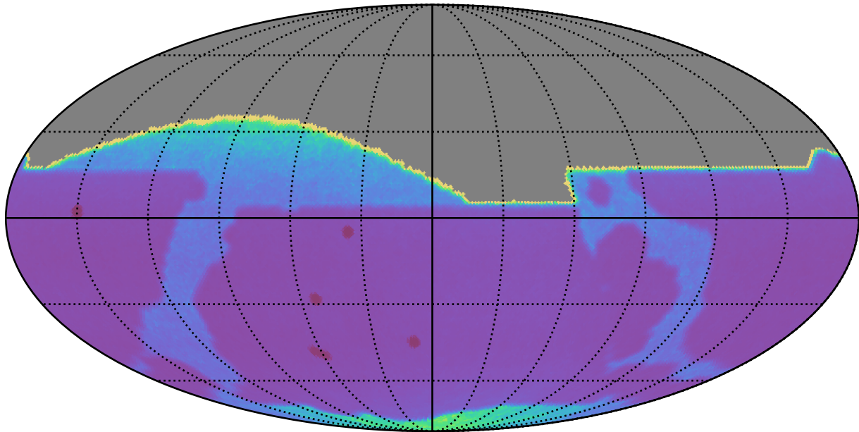
noroll_v3.4_10yrs : Proper Motion Uncert @ 20.5
