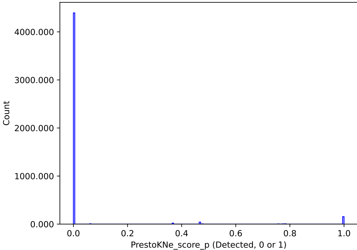
noroll_v3.4_10yrs : PrestoKNe_score_p
