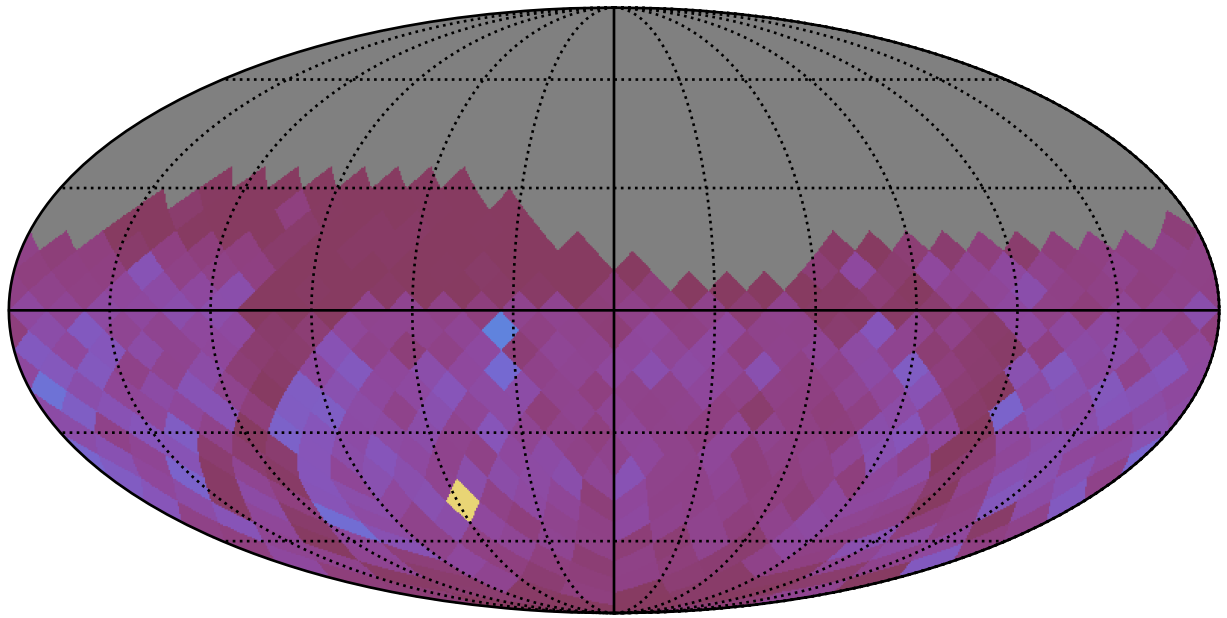
noroll_v3.4_10yrs dm 21 interval 30 RRC Year 1-2: PeriodicStarModulationMetric
