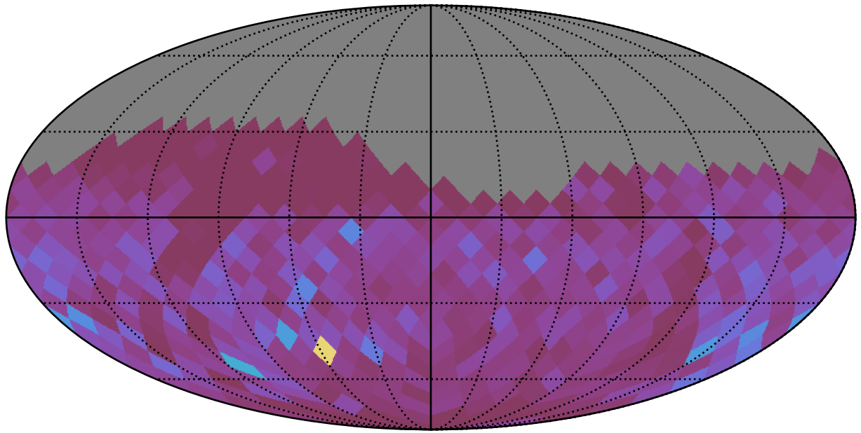
noroll_v3.4_10yrs dm 21 interval 15 RRc Year 1-2: PeriodicStarModulationMetric
