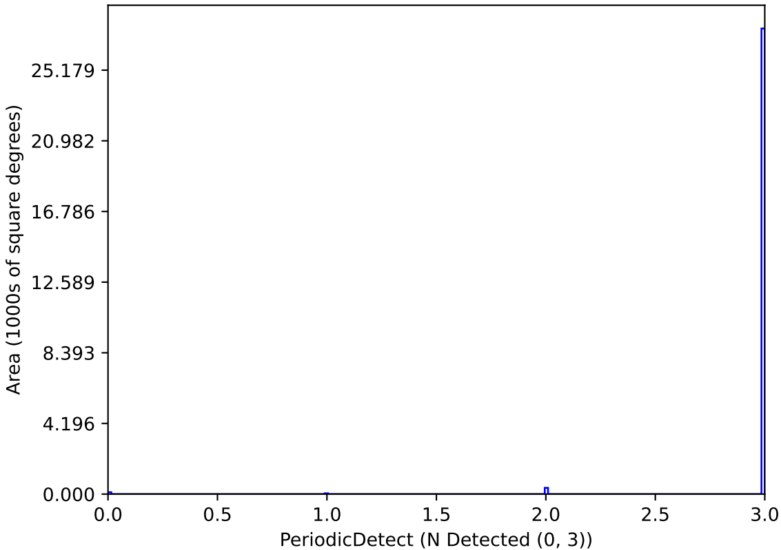
noroll_v3.4_10yrs P_2.0_Mag_21_Amp_0.05-0.1-1: PeriodicDetect
