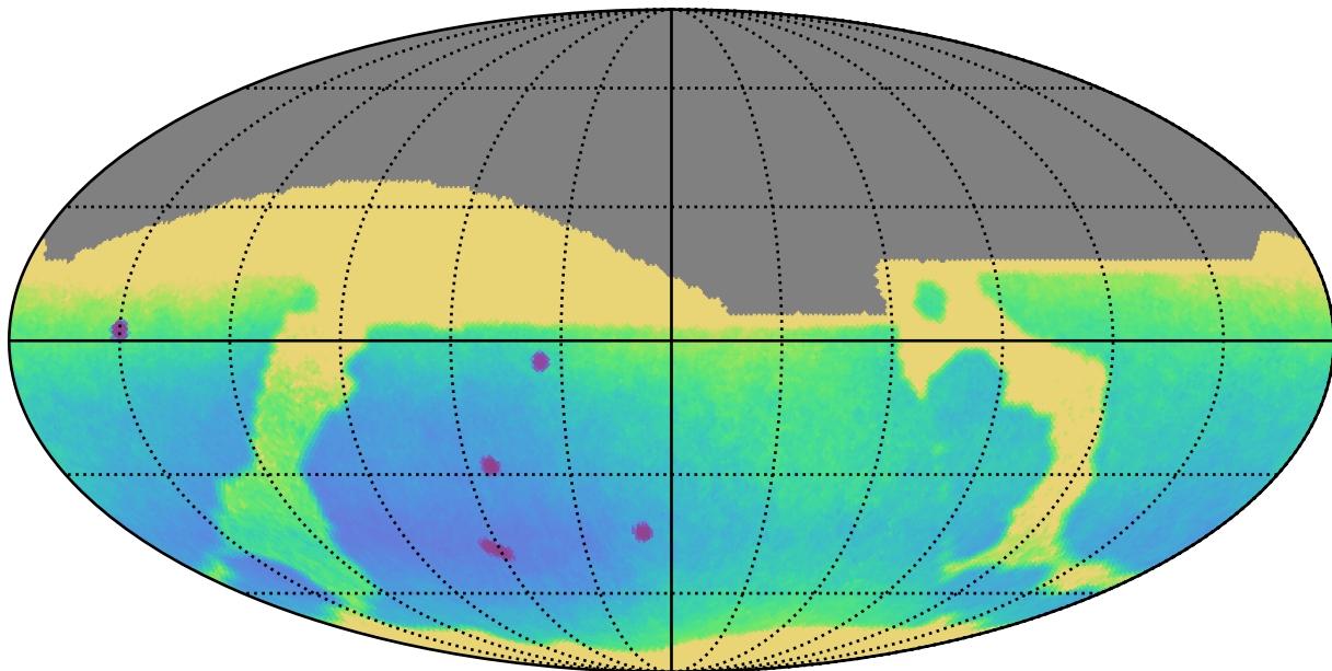
noroll_v3.4_10yrs : Parallax Uncert @ 24.0
