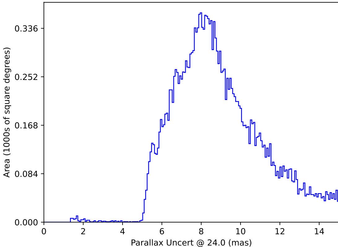
noroll_v3.4_10yrs : Parallax Uncert @ 24.0
