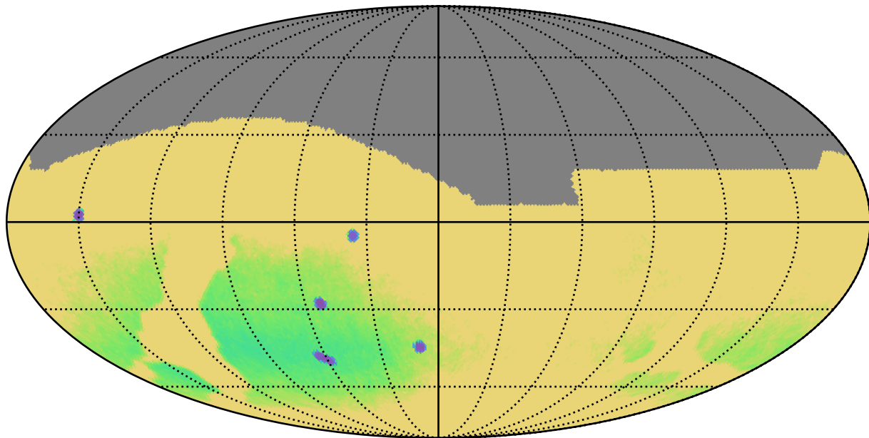
noroll_v3.4_10yrs : Parallax Uncert @ 22.4
