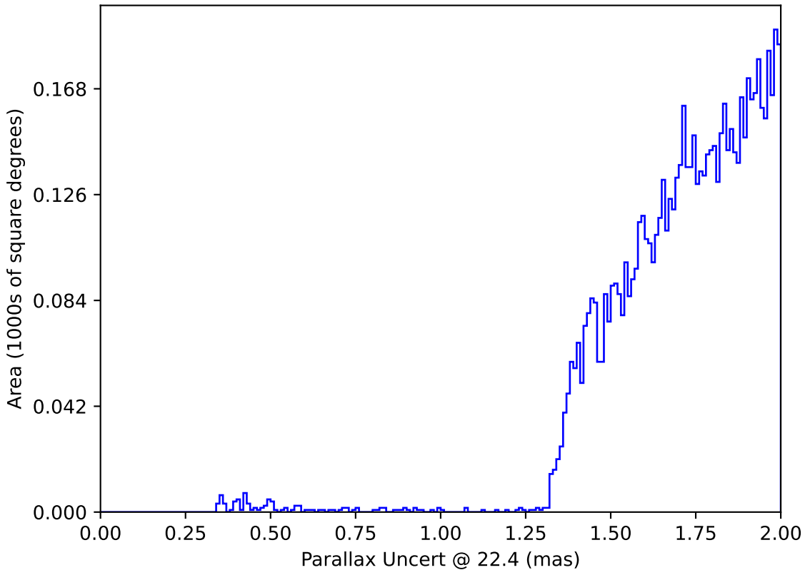
noroll_v3.4_10yrs : Parallax Uncert @ 22.4
