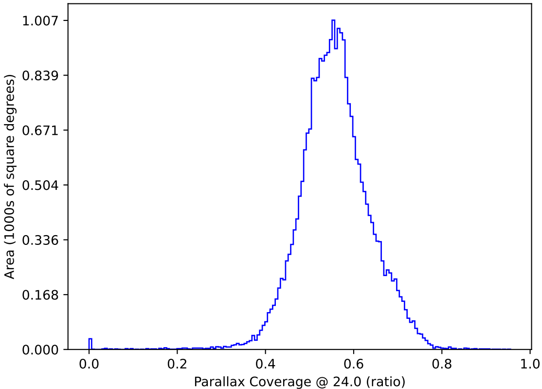
noroll_v3.4_10yrs : Parallax Coverage @ 24.0
