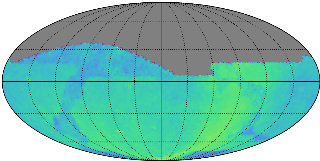
noroll_v3.4_10yrs : Parallax Coverage @ 22.4
