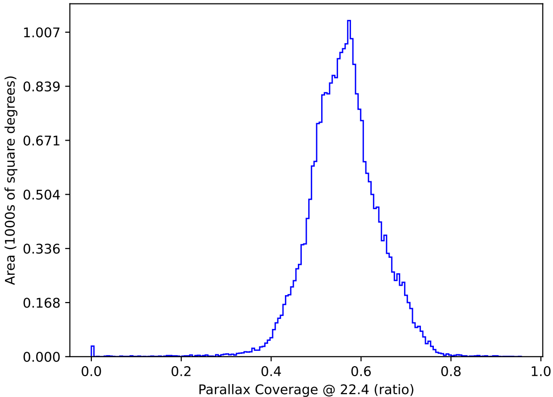
noroll_v3.4_10yrs : Parallax Coverage @ 22.4
