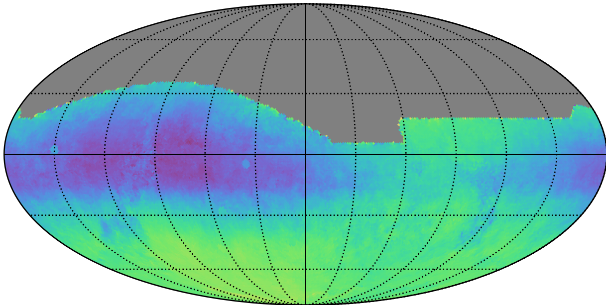
noroll_v3.4_10yrs : Parallax-DCR degeneracy @ 24.0
