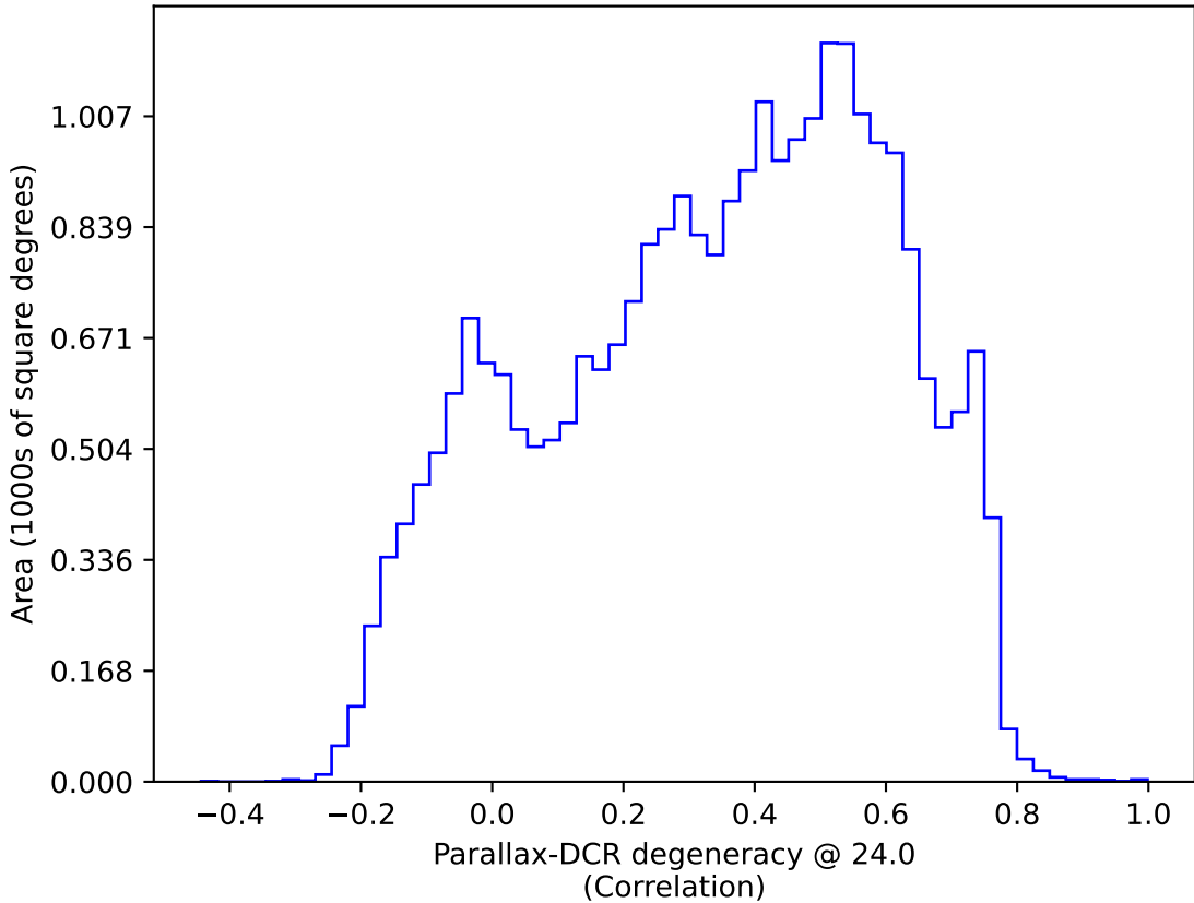
noroll_v3.4_10yrs : Parallax-DCR degeneracy @ 24.0
