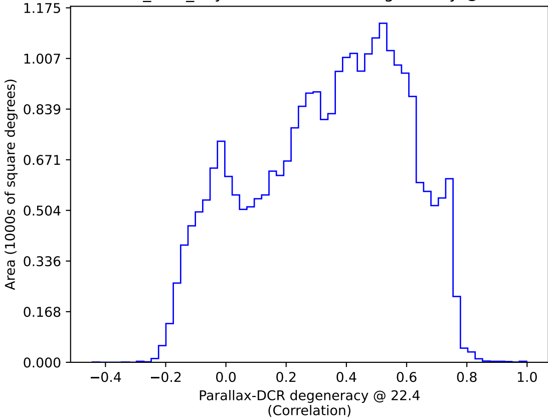
noroll_v3.4_10yrs : Parallax-DCR degeneracy @ 22.4
