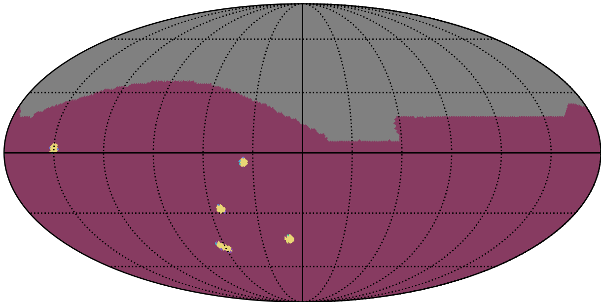
noroll_v3.4_10yrs : NumberOfQuickRevisits
