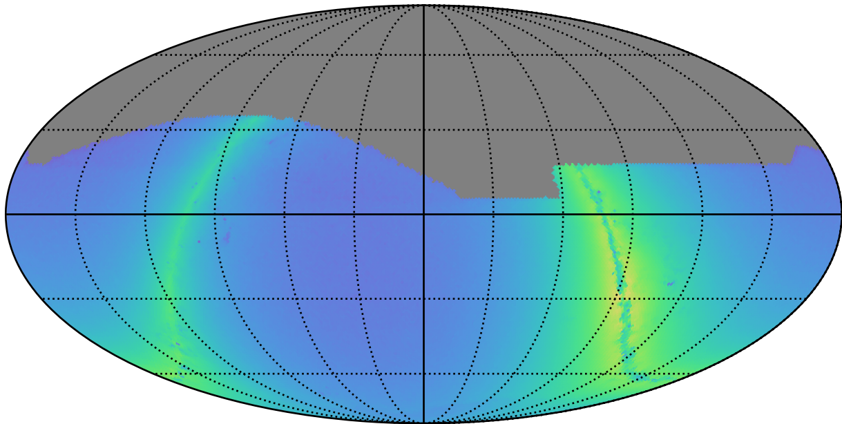
noroll_v3.4_10yrs z: Nstars_no_crowding
