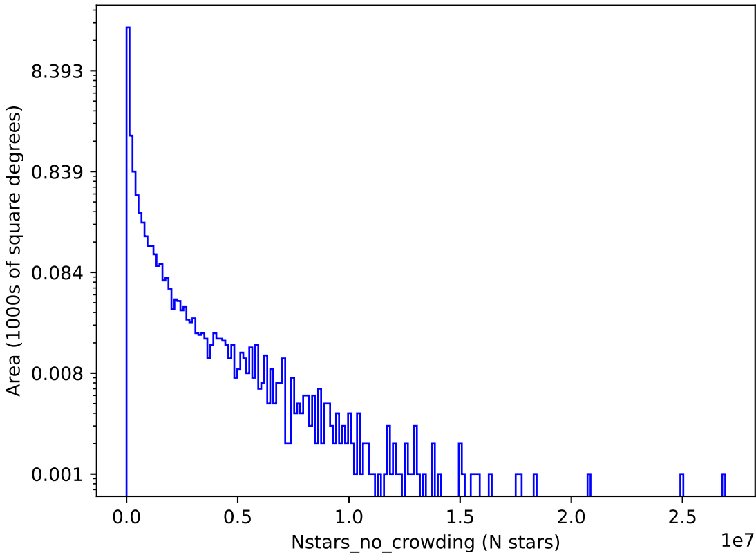
noroll_v3.4_10yrs z: Nstars_no_crowding
