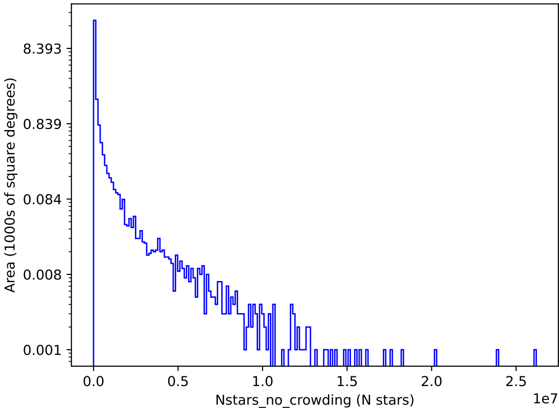
noroll_v3.4_10yrs y: Nstars_no_crowding
