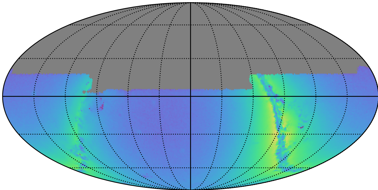
noroll_v3.4_10yrs u: Nstars_no_crowding
