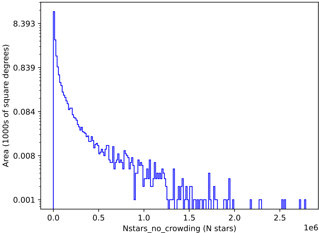
noroll_v3.4_10yrs u: Nstars_no_crowding
