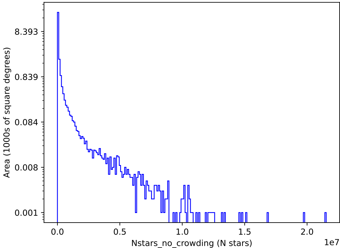
noroll_v3.4_10yrs r: Nstars_no_crowding
