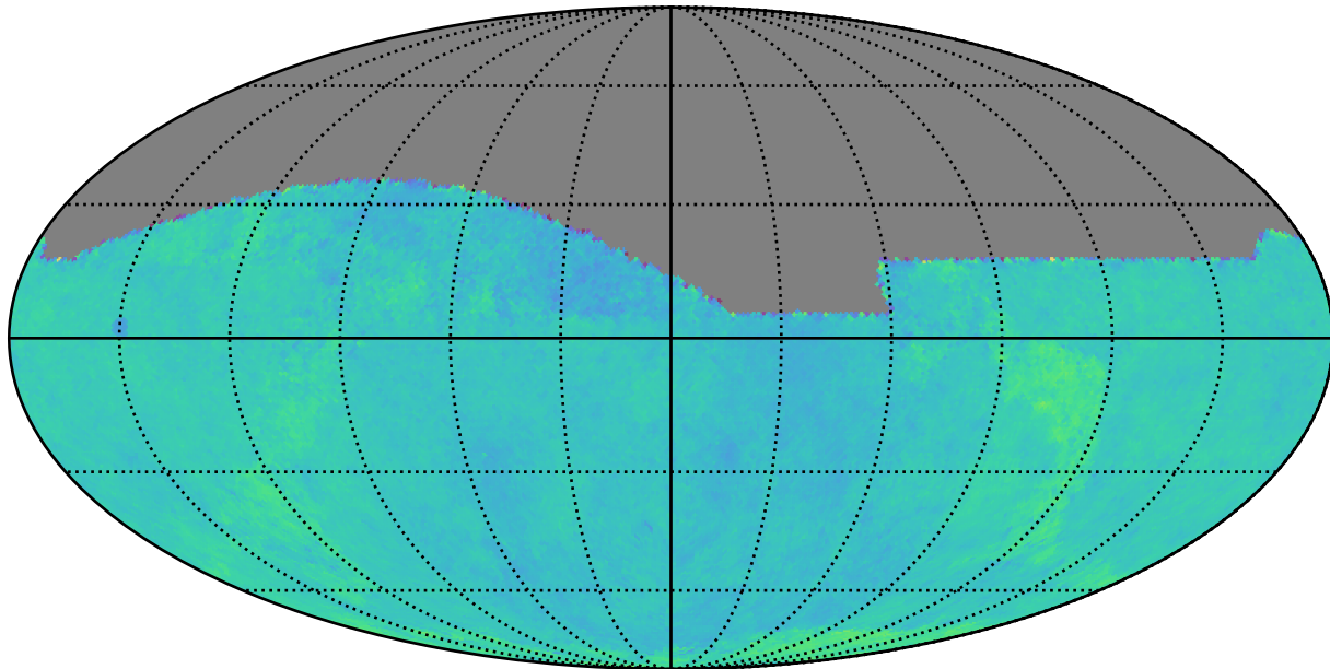
noroll_v3.4_10yrs : Normalized Proper Motion Uncert @ 24.0
