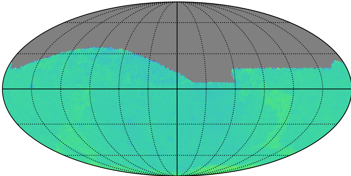
noroll_v3.4_10yrs : Normalized Proper Motion Uncert @ 20.5
