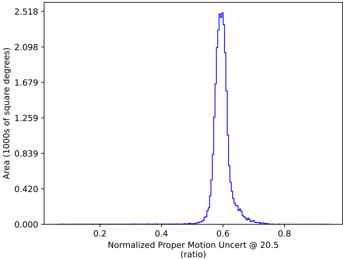
noroll_v3.4_10yrs : Normalized Proper Motion Uncert @ 20.5
