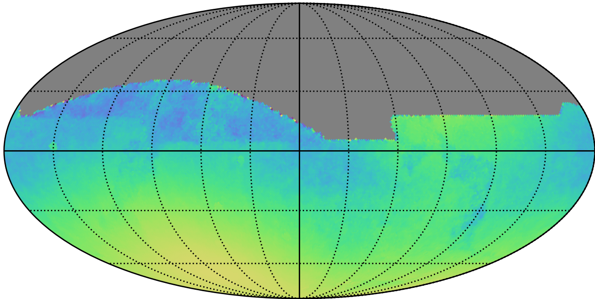
noroll_v3.4_10yrs : Normalized Parallax Uncert @ 24.0
