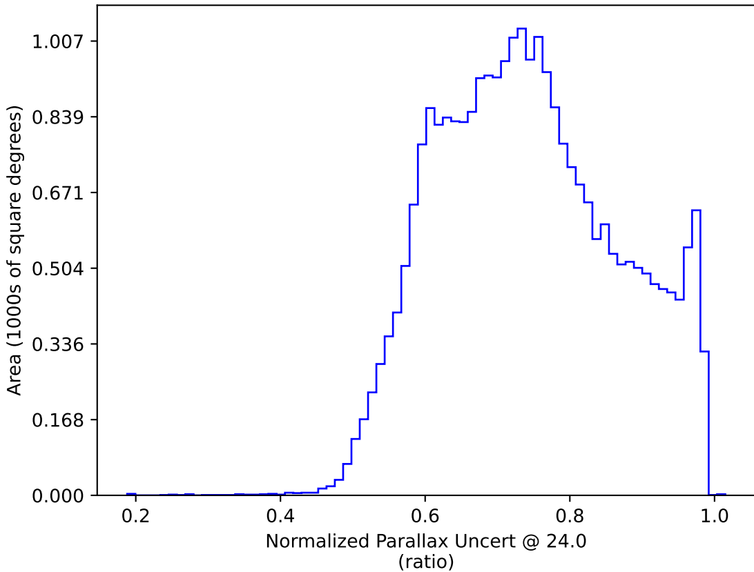
noroll_v3.4_10yrs : Normalized Parallax Uncert @ 24.0
