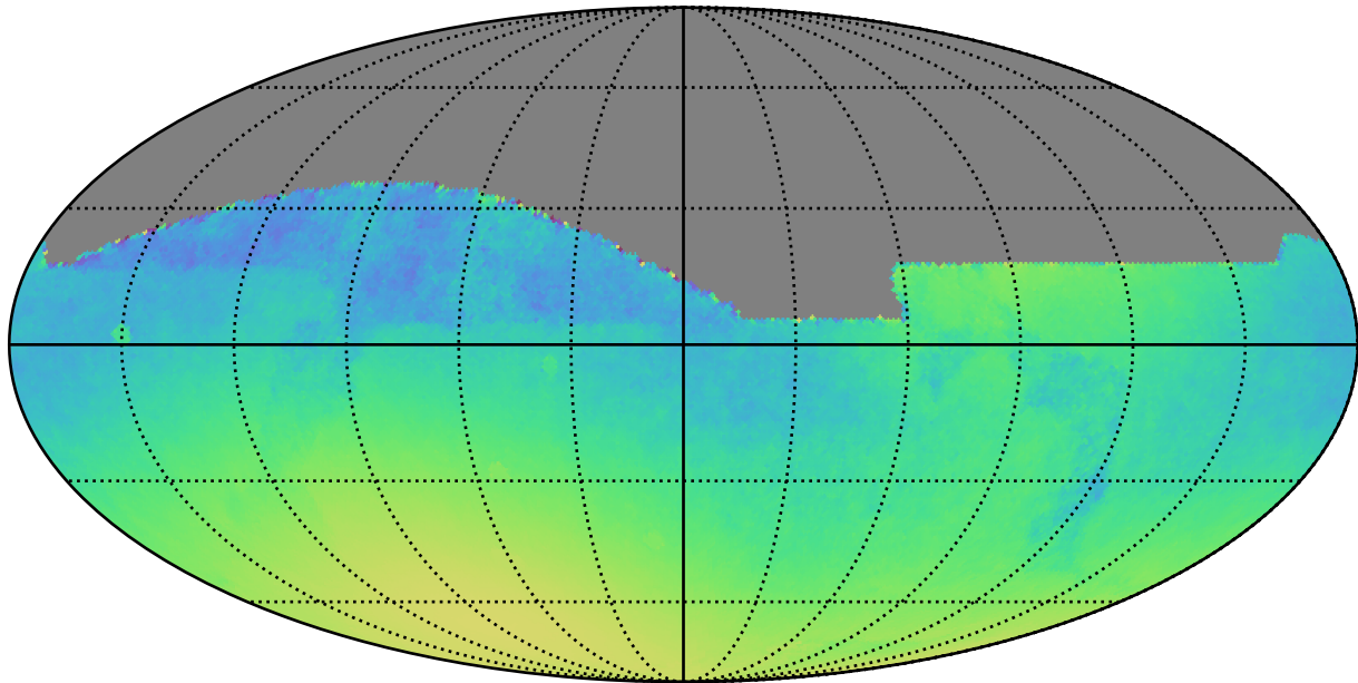
noroll_v3.4_10yrs : Normalized Parallax Uncert @ 22.4
