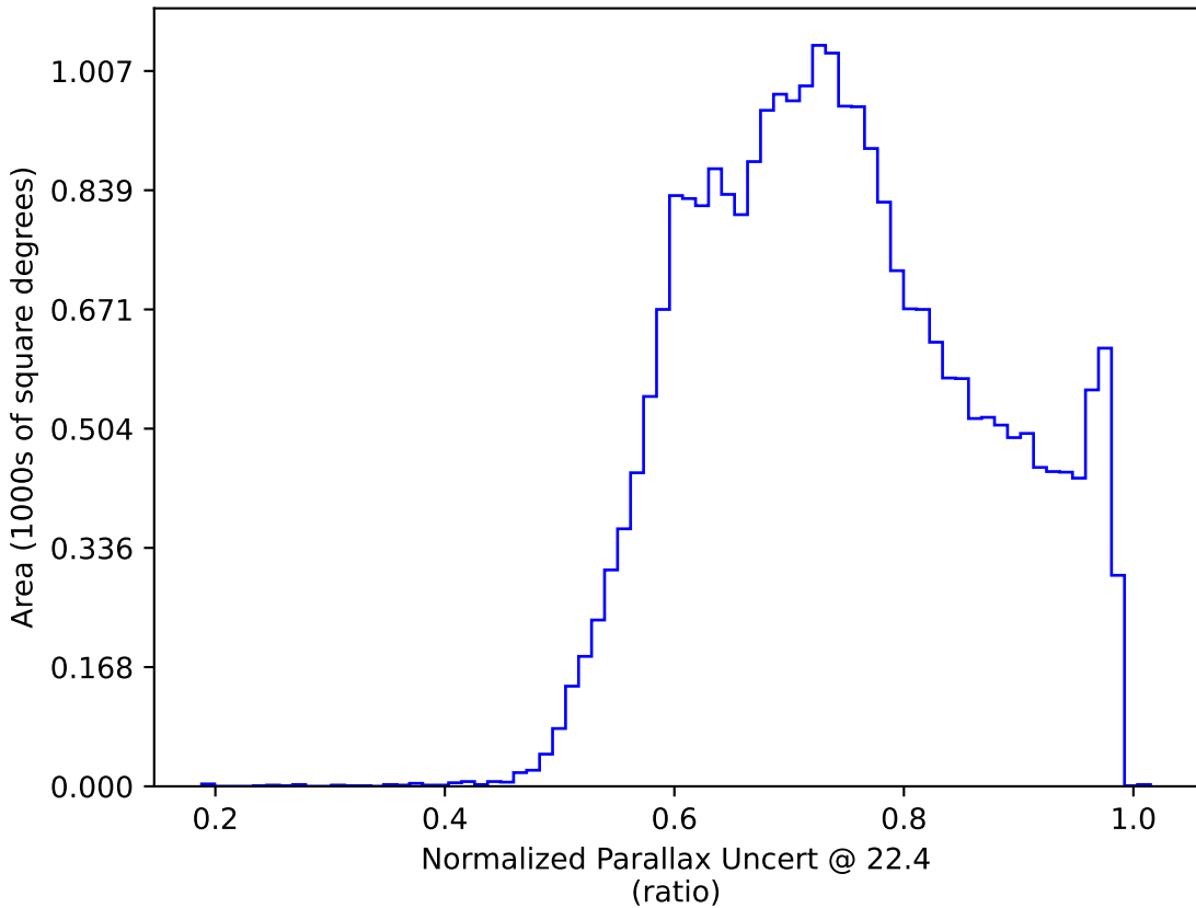
noroll_v3.4_10yrs : Normalized Parallax Uncert @ 22.4
