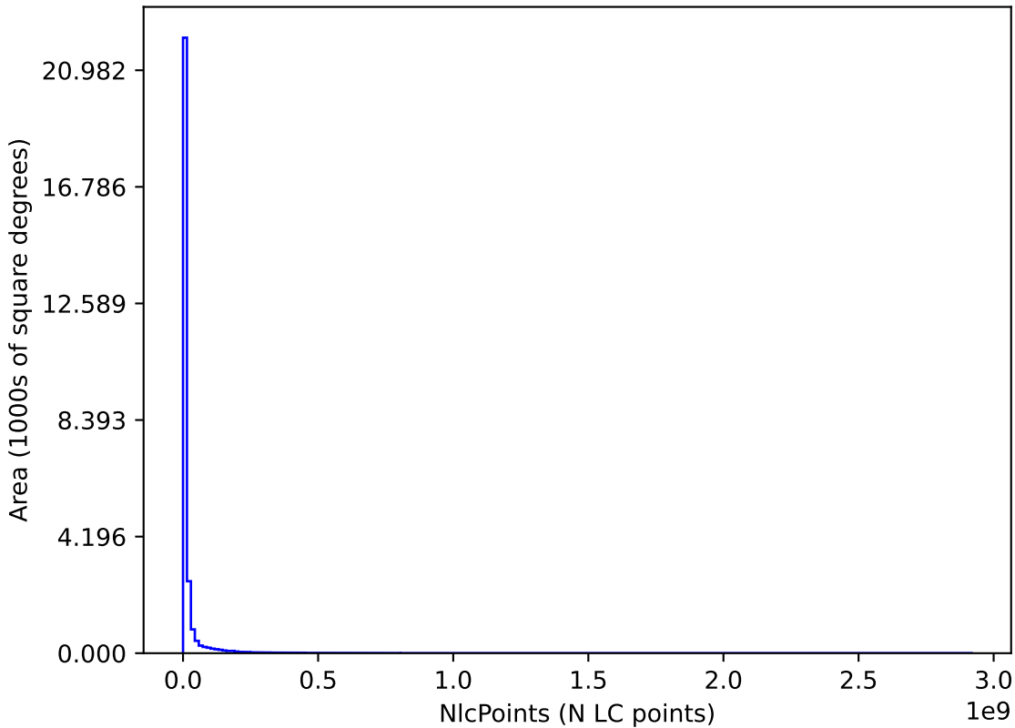
noroll_v3.4_10yrs : NlcPoints
