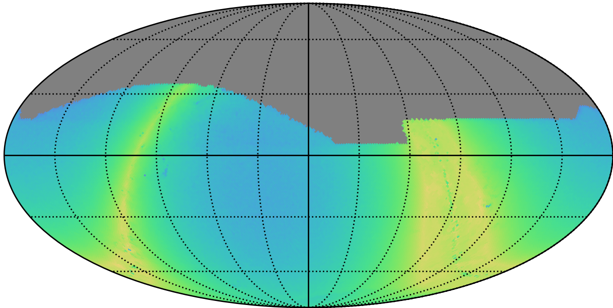
noroll_v3.4_10yrs z: N stars to Precision 0.20
