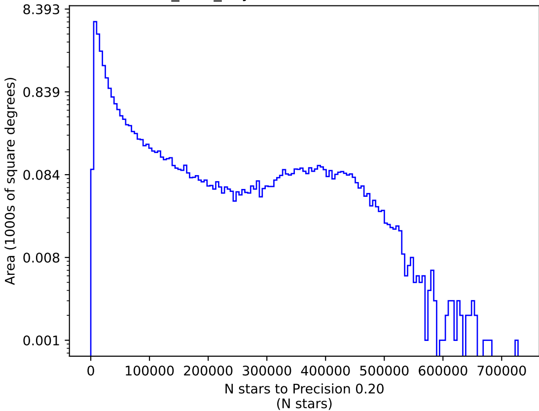
noroll_v3.4_10yrs z: N stars to Precision 0.20
