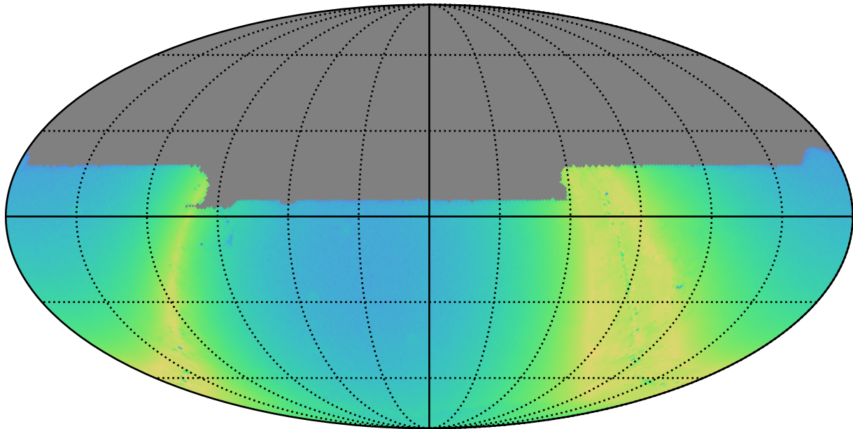
noroll_v3.4_10yrs y: N stars to Precision 0.20
