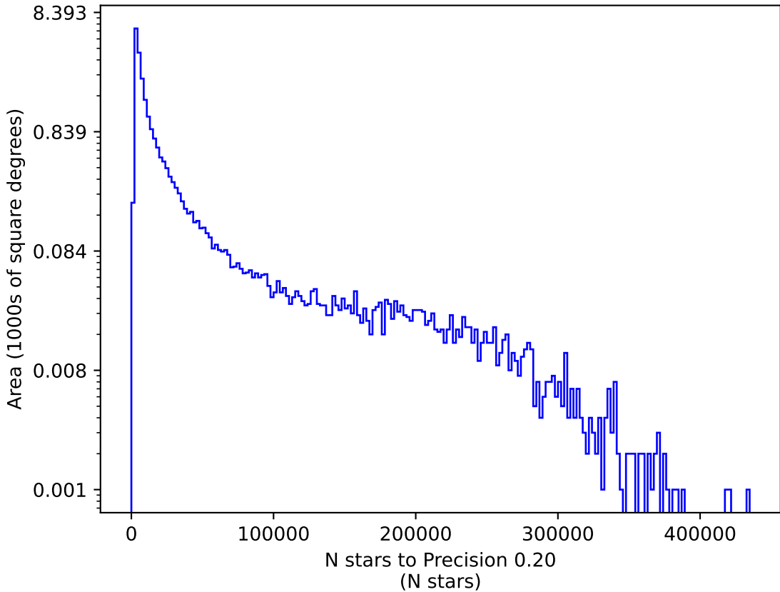
noroll_v3.4_10yrs u: N stars to Precision 0.20
