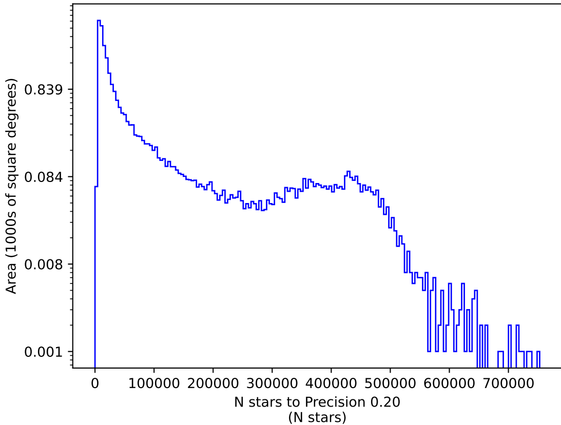
noroll_v3.4_10yrs r: N stars to Precision 0.20
