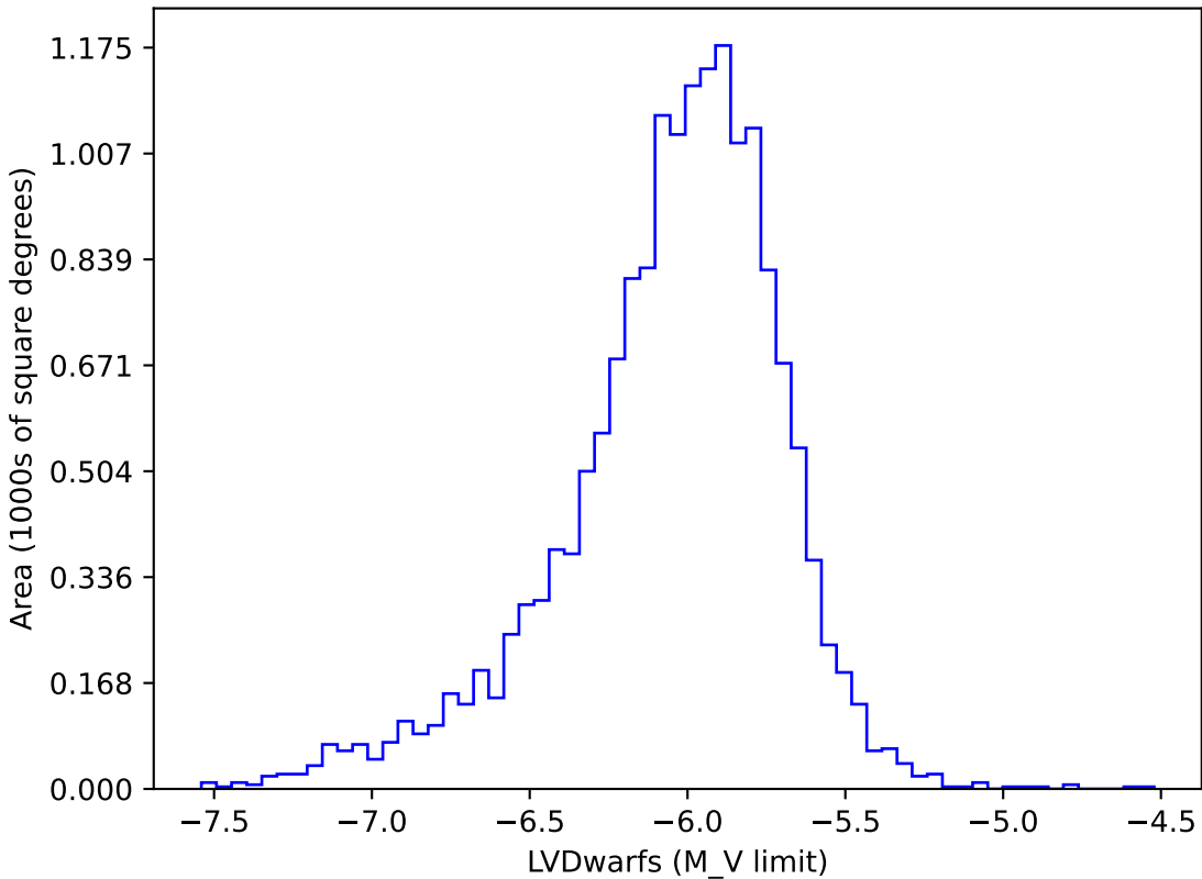
noroll_v3.4_10yrs gi: LVDwarfs
