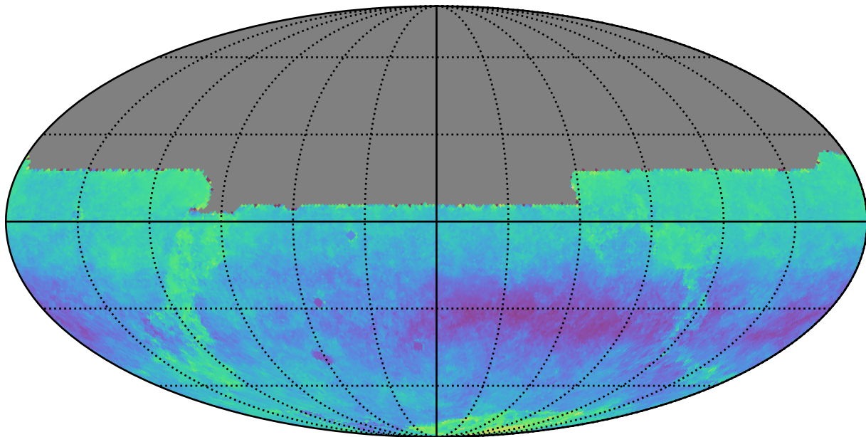
noroll_v3.4_10yrs y: Kuiper rotSkyPos
